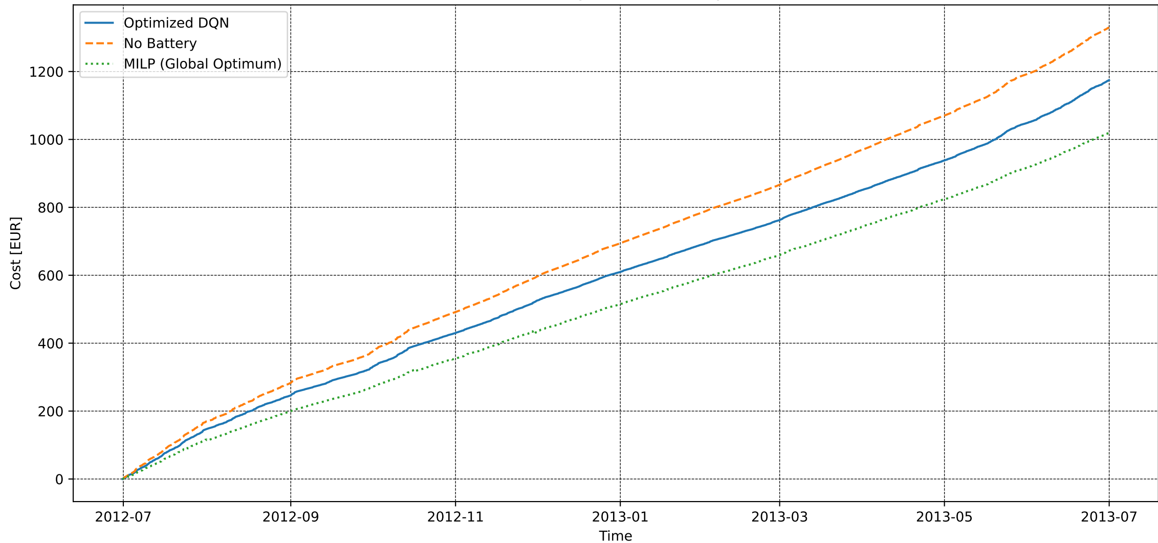
User 247 - Extended Convergence - Electricity Cost [DQN vs MILP]
